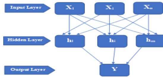
Figure 2:MLP Architecture
