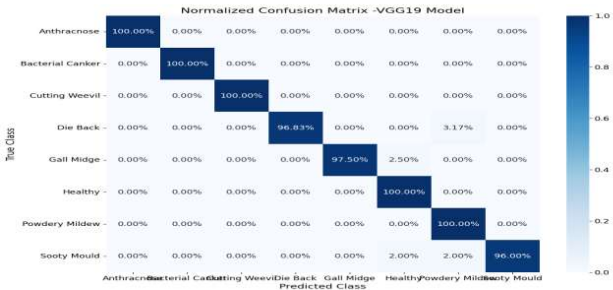
Figure 8 Confusion matrix of VGG19 Model
